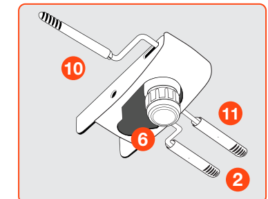
R3 ROCKING TILT
